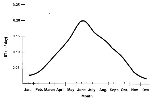
Fig. 6. Seasonal ET rates in a citrus orchard, San Joaquin Valley.
