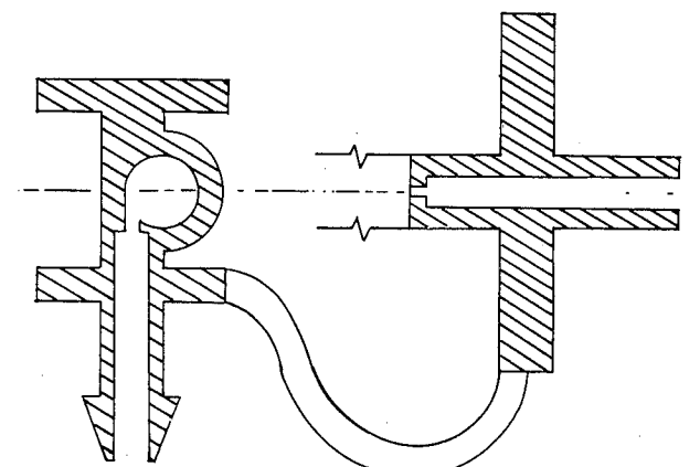
Fig. 4. Cross-section of vortex type emitter showing turbulent-flow chamber.
