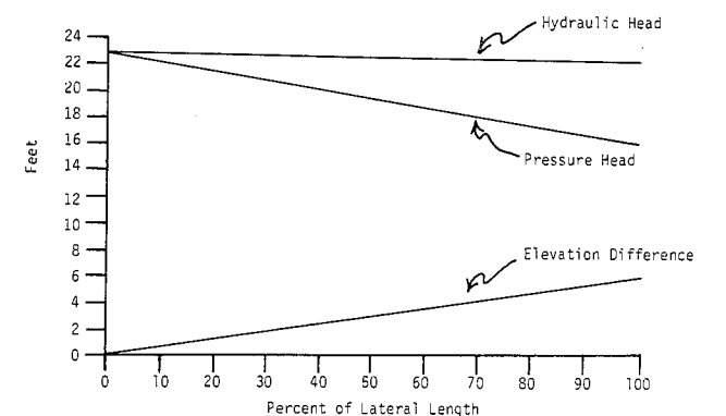
Fig. 7. Distribution of pressure head and hydraulic head and elevation changes in lateral.
