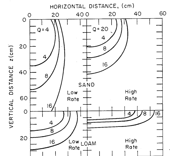
Fig. 2. Water distribution profiles in soils of two textures at two rates of water application, Q = 1 and 5 gallons per hour (4 and 20 liters per hour). The numbers on the curves refer to total quantities of water applied. (Redrawn from Bresler, 1977.)
