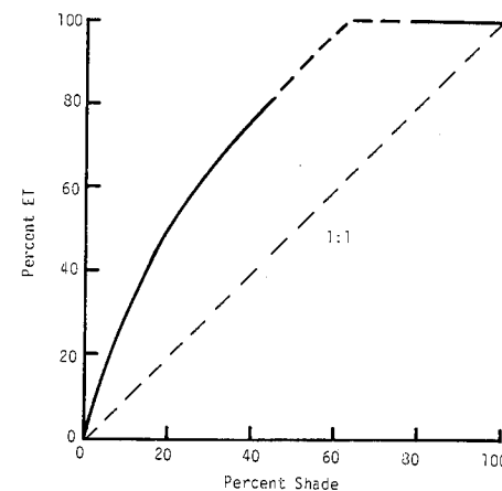
Fig. 8. Relationship between percent ground area shaded by tree canopy in midsummer and ET of drip irrigated young trees as a percent of ET of mature orchards. NOTE: Dashed portion of upper line indicates portions of the relationship where no experimental data are yet available.
