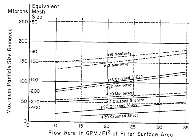
Fig. 1. Filtration efficiency of different grades and types of sand at various flow rates. SOURCE: Yardney, Water Management Products Division.
