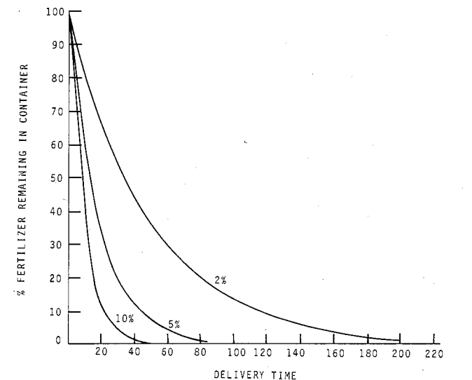
Fig. 2. Calculated fertilizer application curves for different flow rates.*
