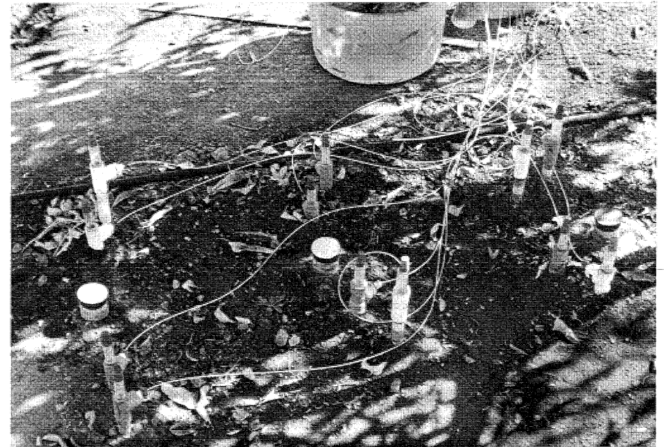
Tensiometers and neutron probe access tubes in place to monitor soil water levels.
