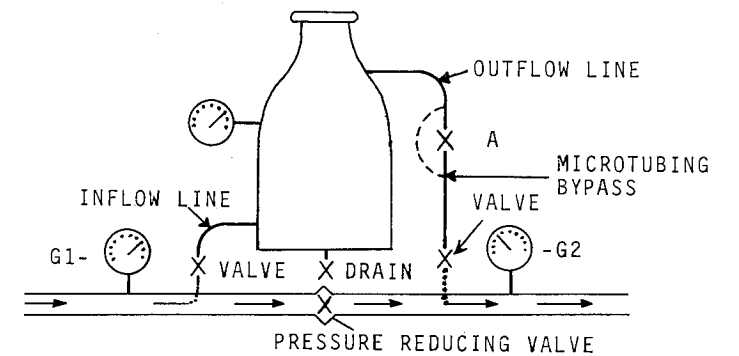
Fig. 1. Schematic diagram of a pressure differential applicator.
