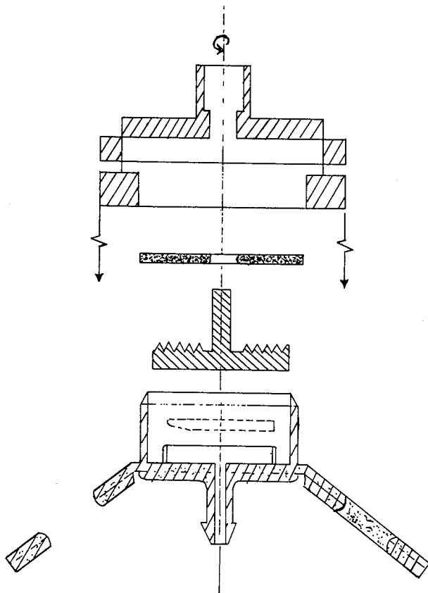
Fig. 5. Cross-section of pressure-compensating emitter with flexible diaphragm to regulate flow.
