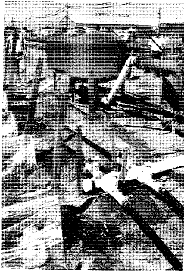
Sand filters being used in drip irrigation of tomatoes.
