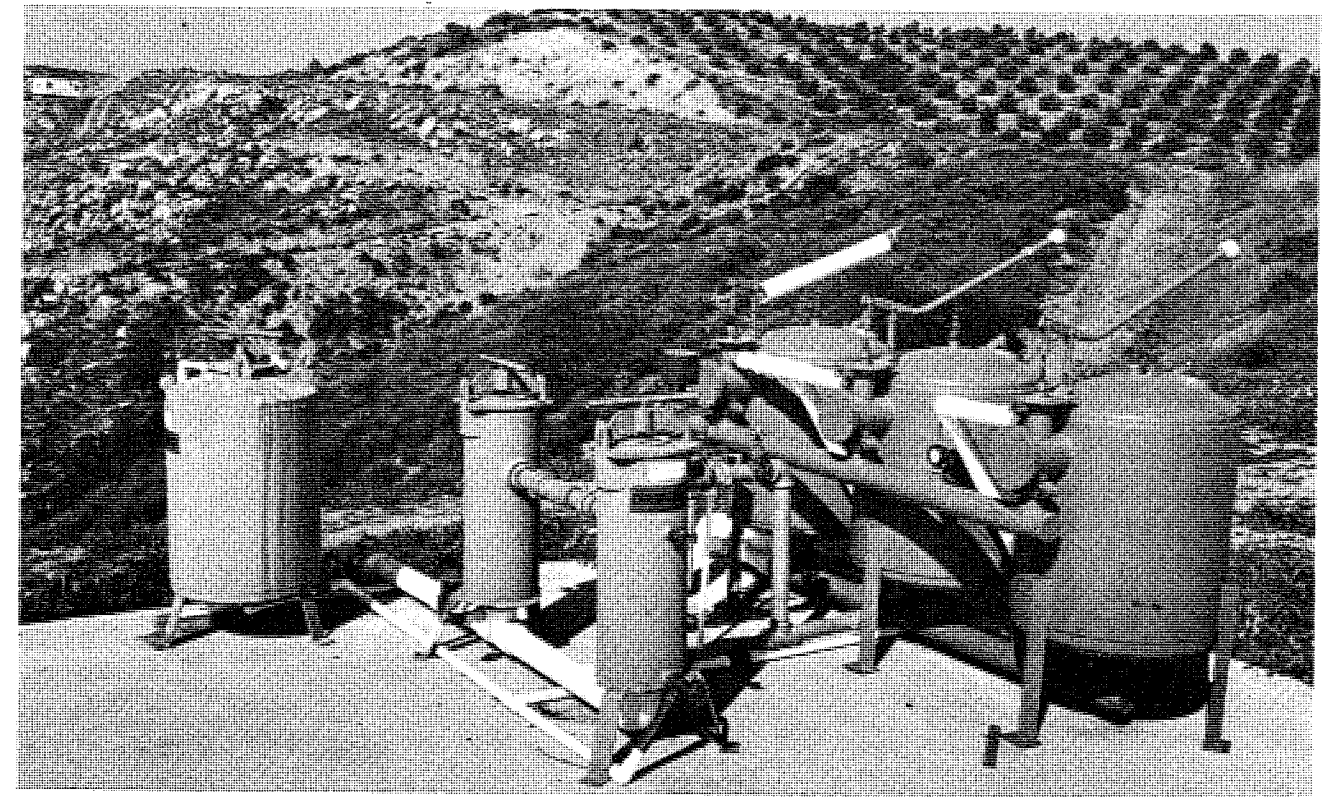
Typical drip irrigation control head.
