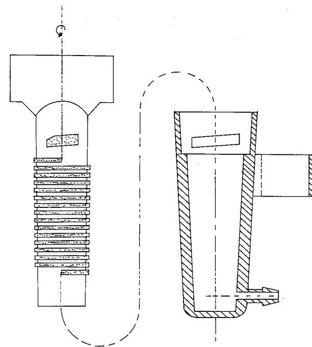
Fig. 2. Cross-section of typical long path emitter.
