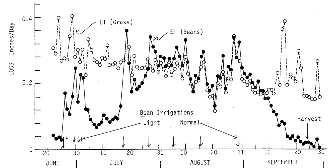
Fig. 2. Daily ET data for beans and grass measured using 2 lysimeters 20 feet in diameter. Davis, California, 1968. Unpublished data from W.O. Pruitt.
