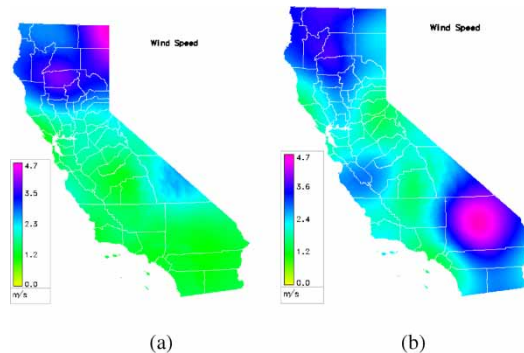
Figure 5. Two typical wind speed interpolations, for a calm 5 and a windy day. (a) 2005/12/21 calm (b) 2005/06/18 windy.
